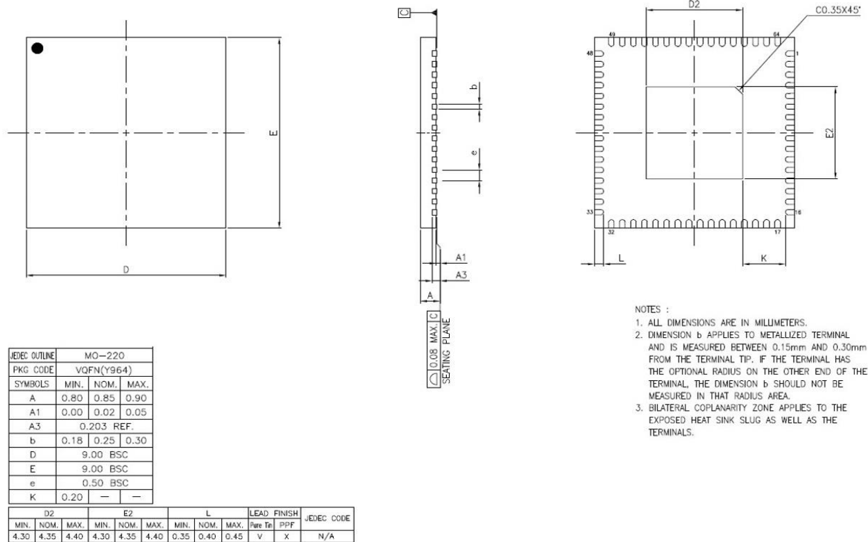
Figure 32 - 64 Pin QFN Package Details
