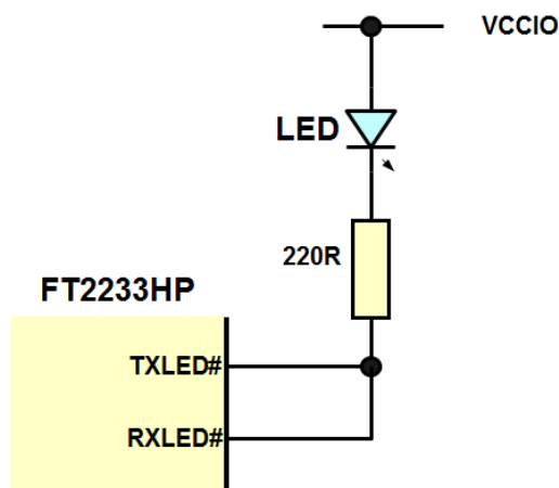
Figure 25 – Single LED UART Configuration
