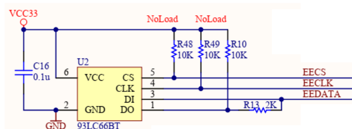
Figure 33 - EEPROM Interface
