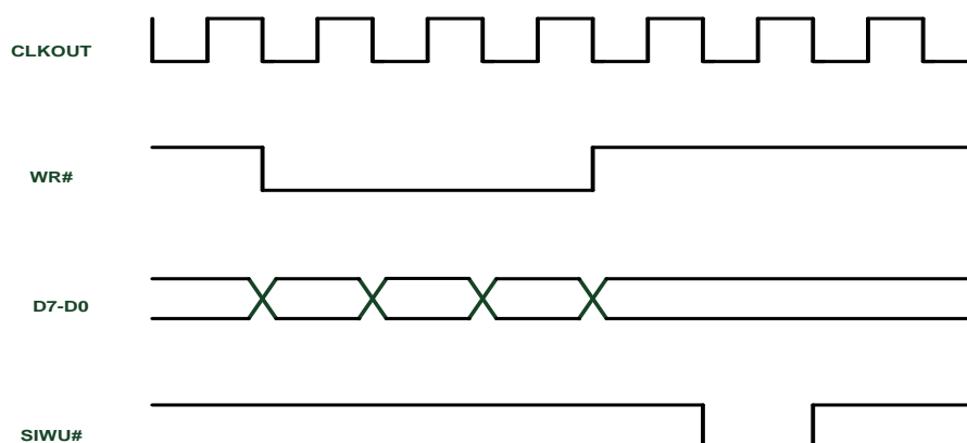
Figure 26 – Using SIWU#
